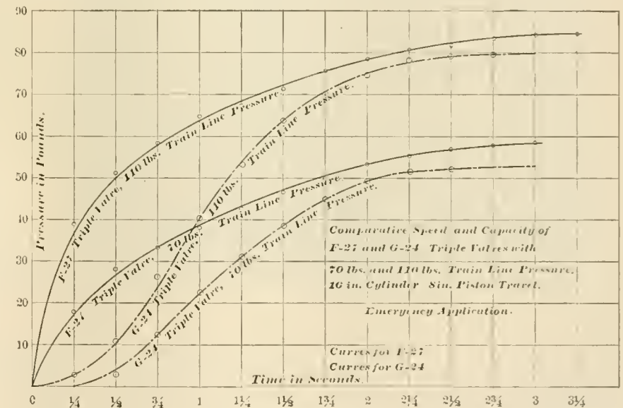
CURVES SHOWING VALUES OF PLAIN AND QUICK ACTION TRIPLES FOR TENDER BRAKES.
